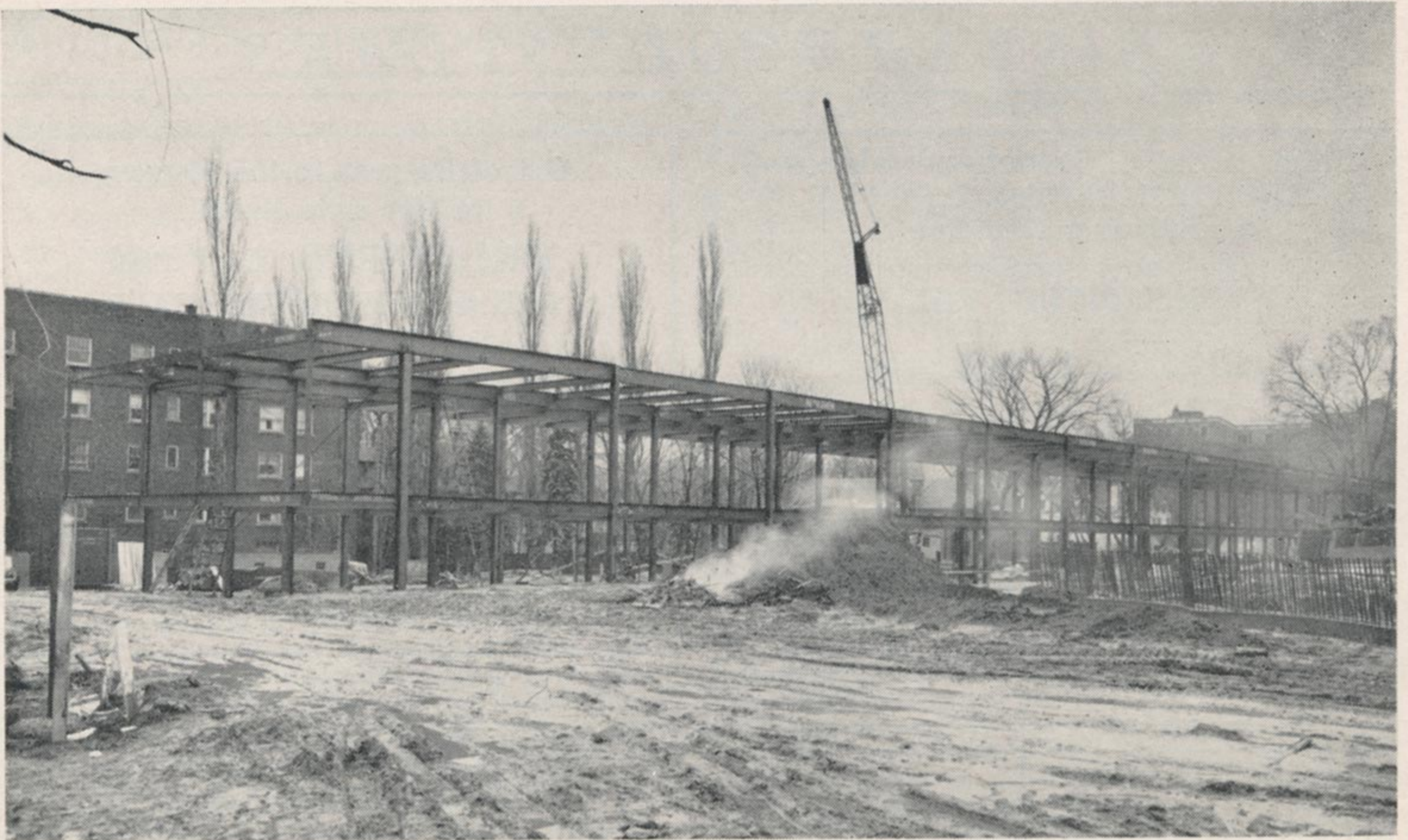
Steel super-structure of Religious School and Temple Office Building as viewed from Delaware Avenue at Barker.
